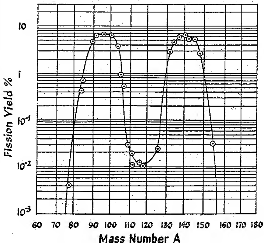
Figure 4—Mass Distribution of Fission Products.
